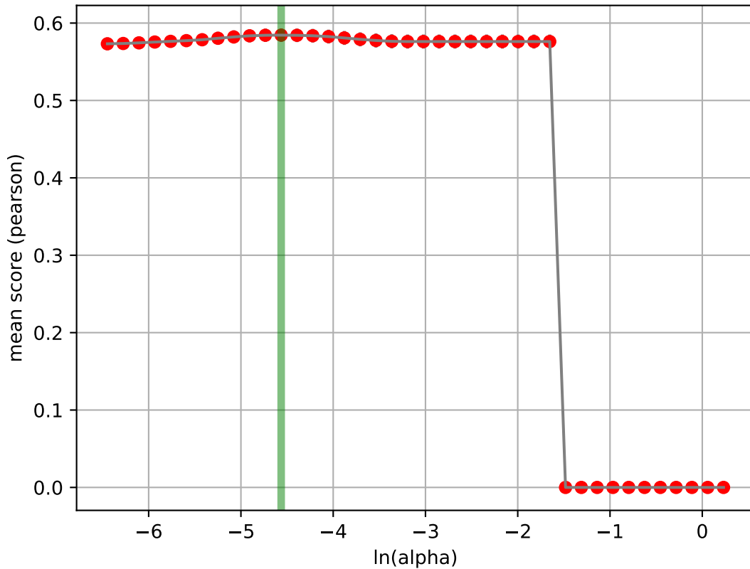
Mean scores (pearson) across alphas for Kfold=10
